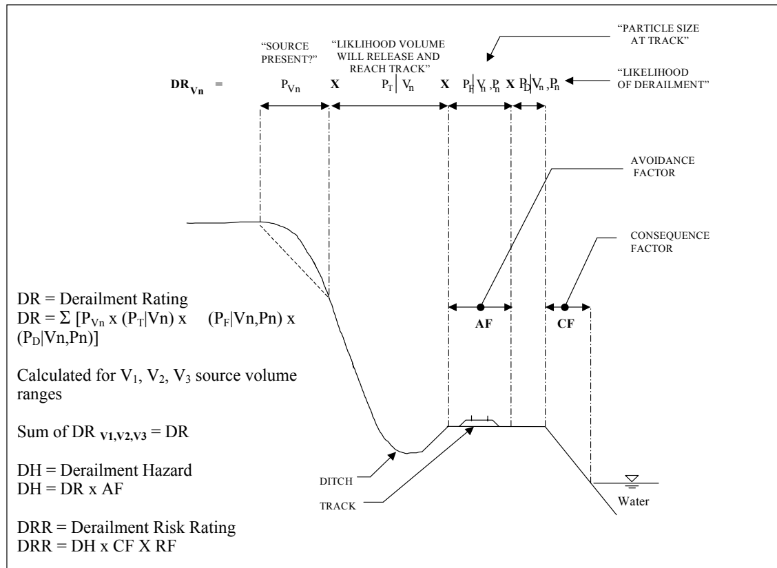
Figure 3. Schematic Illustration of Derailment Rating (DR) Calculation
